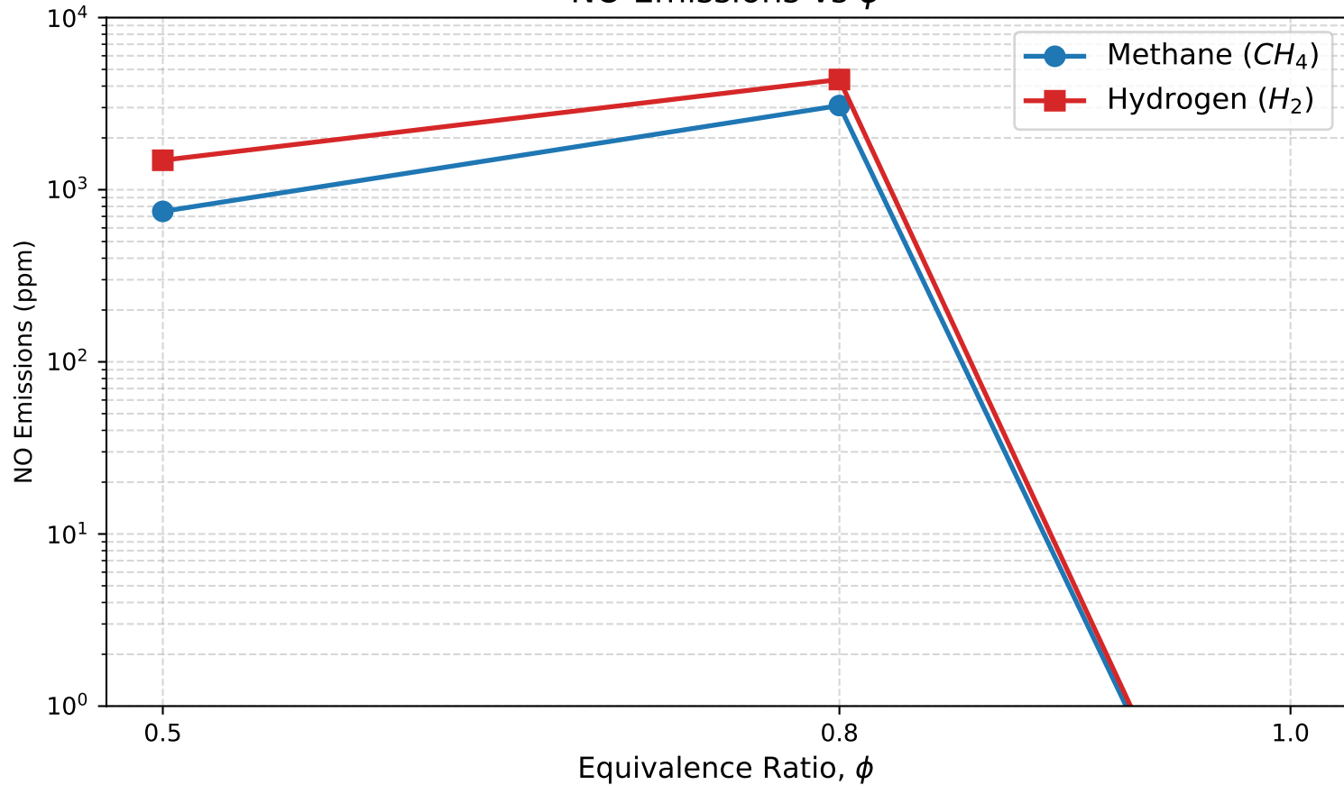
NO Emissions vs \phi
